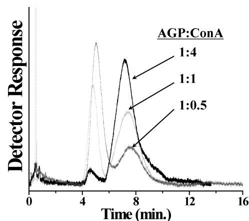
Figure 4. The superimposed fractograms of AGP and AGP bound ConA obtained by varying mass ration of AGP/ConA as 1:0.5, 1:1, and 1:4. Injection amount of AGP was fixed as 1 \mu g except for same ratio 1:0.5 (2 \mu g of AGP was used in this case, but the entire fractograms were area-normalized to compare the relative distribution of each component).
