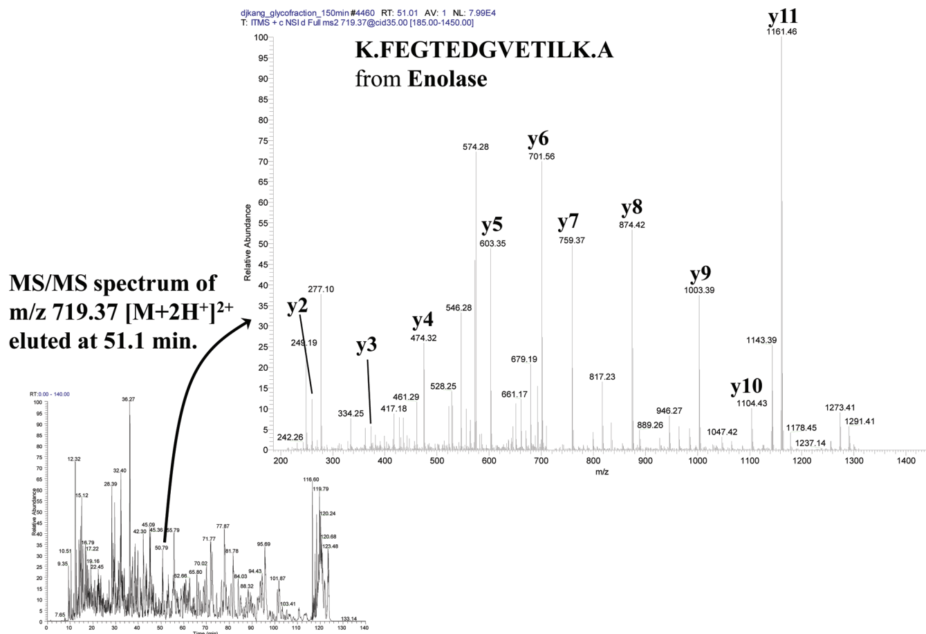
Figure 6. Precursor scan MS spectra at 51.1 min during RPLC-ESI-MS-MS run and the corresponding CID spectra of a precursor ion m/z 719.37 [\text{M} + 2\text{H}^+]^{2+} were identified as a peptide of K.FEGTEDGVETILK.A from Enolase (RPLC-ESI-MS-MS run was obtained after the salt step elution with 2 mM \text{NH}_4\text{HCO}_3 )
