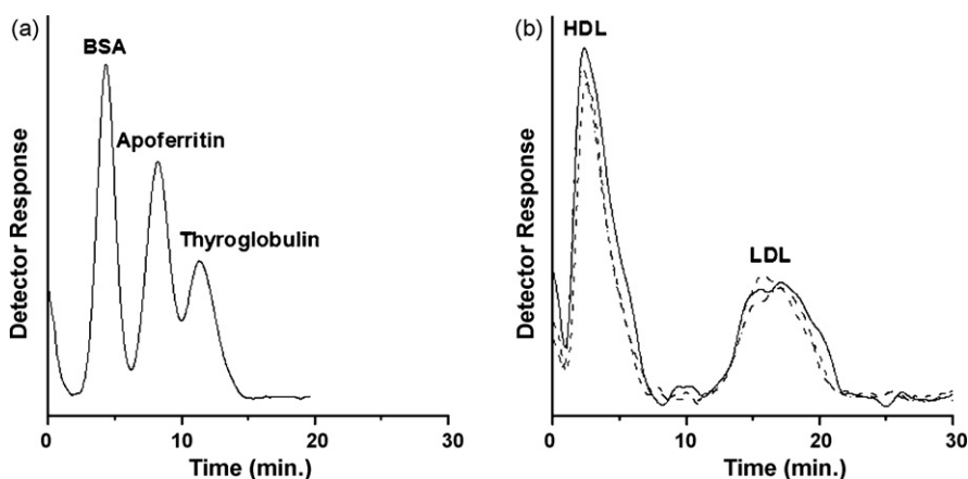
Fig. 3. MxHF5 fractograms of (a) the separation of protein standards (10 \mu g of each standard) at 280 nm and (b) the separation of HDL and LDL particles from a human plasma sample (50 \mu L stained with Sudan Black B) at 600 nm. The outflow rate was 1.7 mL/min and the radial flow rate was 1.3 mL/min for both runs.
