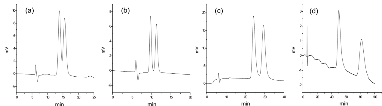
Figure 5. Chromatogram of (a) Tröger base, (b) trans -stilbene oxide, (c) benzoin and (d) warfarin isomers separated on CSP-3. The mobile phase is heptane/2-propanol (90/10 v/v%), the flow rate, 0.01 mL/min, and the UV wavelength, 254 nm.
